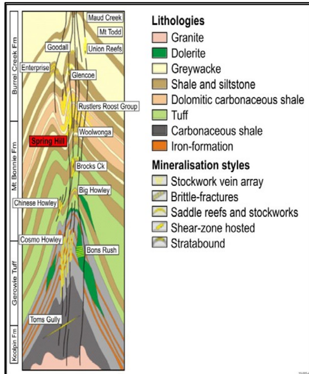
Figure 3: Structural and stratigraphic setting and styles of gold mineralisation in the Pine Creek Inlier (After N. T. Geological Survey)
